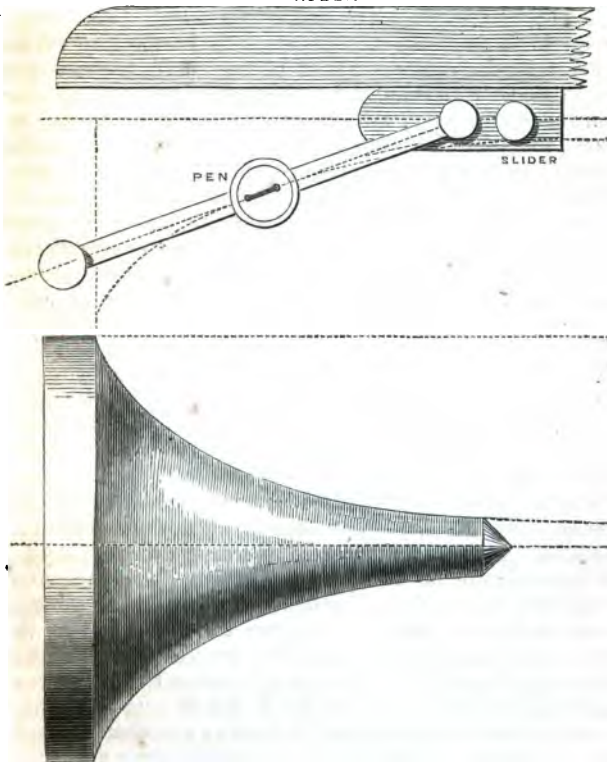
Mode of striking the curve to form the millstone or pivot.
